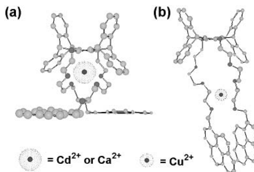
Figure 3. Molecular models showing the proposed structures of 1 in dichloromethane in the presence of (a) \text{Ca}^{2+} or \text{Cd}^{2+} and of (b) \text{Cu}^{2+} .
