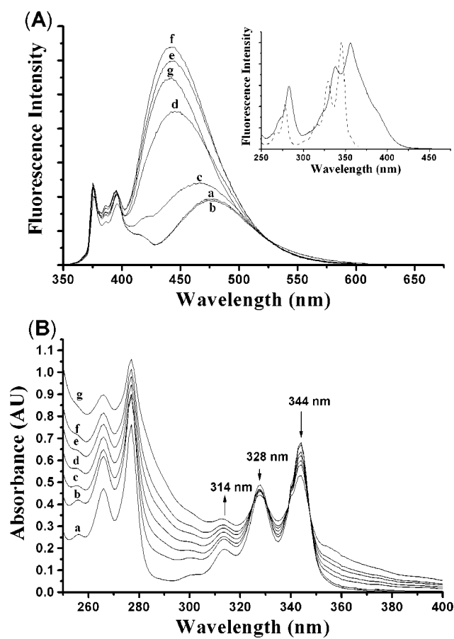
Figure 2. (A) Fluorescence and (B) absorption spectra of 1 in \text{CH}_2\text{Cl}_2 ( 1 \times 10^{-5} M, excitation at 335 nm) in the presence of (a) 0, (b) 1.0, (c) 5.0, (d) 7.0, (e) 9.0, (f) 11.0, and (g) 15 equiv of \text{Cu}(\text{ClO}_4)_2 \cdot 6\text{H}_2\text{O} predissolved in MeCN (0.005 M) and the corresponding change in the excitation spectra (normalized) monitored at 375 (dash) and 440 (full) nm (inset).
