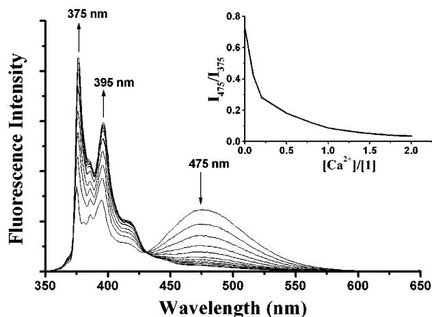
Figure 1. Fluorescence spectra of 1 in \text{CH}_2\text{Cl}_2 ( 1 \times 10^{-5} M, excitation at 335 nm) in the presence of 0, 0.1, 0.2, 0.5, 0.8, 1.0, 1.2, 1.4, 1.6, 1.8, and 2.0 equiv of \text{Ca}(\text{ClO}_4)_2 \cdot 4\text{H}_2\text{O} predissolved in MeCN (0.005 M) and the corresponding change in the I_E/I_M ratio represented by the intensities at 475 ( I_{475} ) and 375 ( I_{375} ) nm (inset).
